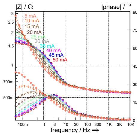
[FIGURE CAPTION] Fig.1. Bode impedance diagrams durin ORR in alkaline solution
